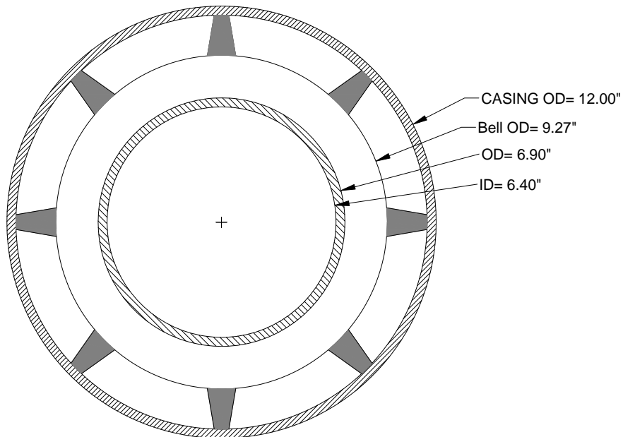
6" CL350 DIP in 12" Steel Casing
