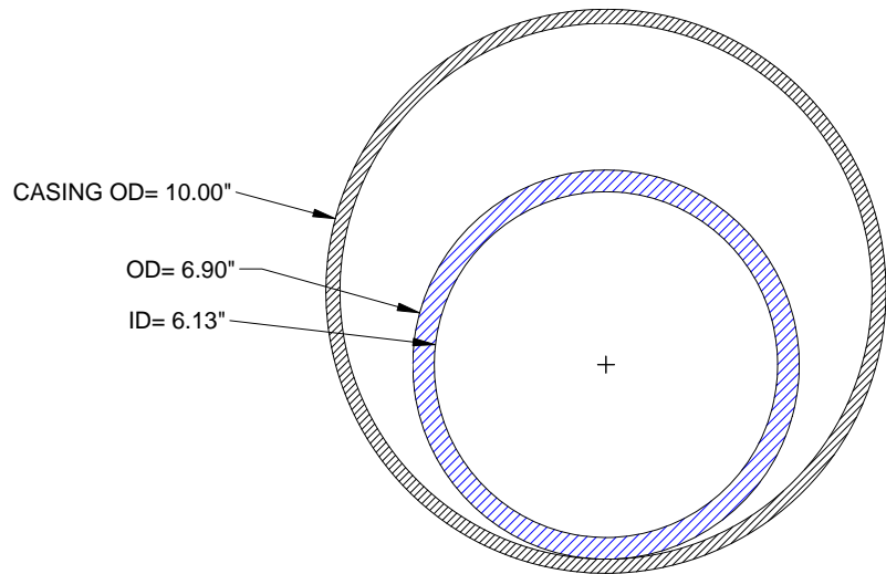
6" DR 18 Fusible C-900® in 10" Steel Casing
